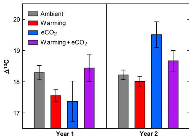
Fig. 4 Effects of elevated CO 2 (eCO 2 ) and warming on Bromus tectorum leaf \Delta^{13}\text{C} in Year 1 and Year 2. Larger \Delta^{13}\text{C} values indicate more discrimination against ^{13}\text{C} (reflecting an increase in the leaf-internal CO 2 concentration). Error bars are \pm 1 SE. See Table 1 for statistical results and Figure S4 for \Delta^{13}\text{C} results within each competition treatment.
