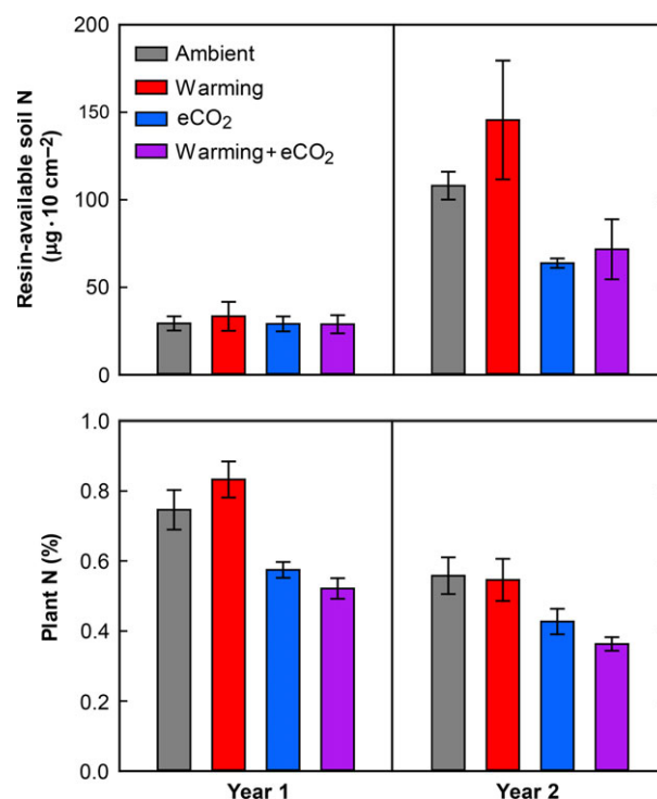
Fig. 5 Effects of elevated CO 2 (eCO 2 ) and warming on resin-available inorganic soil N (measured in low-competition subplots) and plant tissue N (averaged across competition treatments). Note that resin probe incubation period was longer in Year 1 than Year 2, to match a longer Bromus tectorum growing season (see Fig. 2), and caution should be used in comparing absolute values across years. Error bars are \pm 1 SE. See Table 1 for statistical results and Figure S5 for plant N results within each competition treatment.
